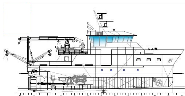
New Coast research vessel (Delivery 2019)
